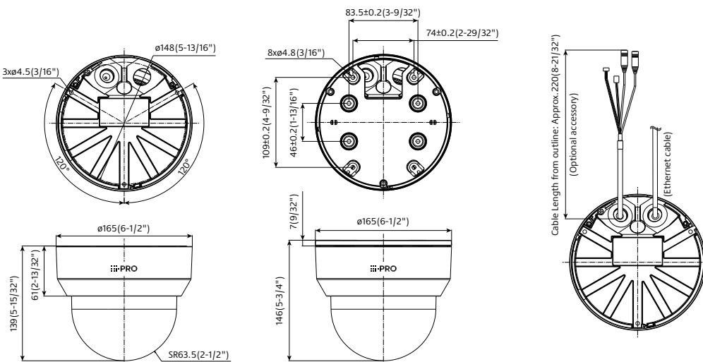
With Attachment plate & Attachment cover
