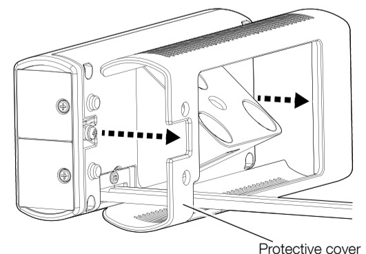
Protective cover
